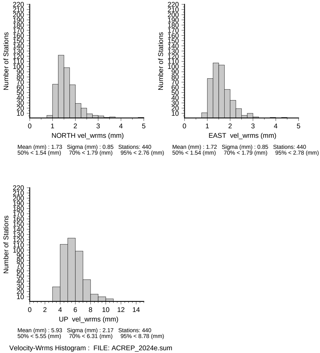
Figure 2: Histogram of the weighted root-mean-square (WRMS) scatter of daily position estimates of sites used more than five times for 2024 after removing linear trends and eliminating gross outliers (5 times WRMS scatter). The median scatters are similar to last year, with 1.5, 1.5 mm horizontal, and 5.6 mm vertical.
