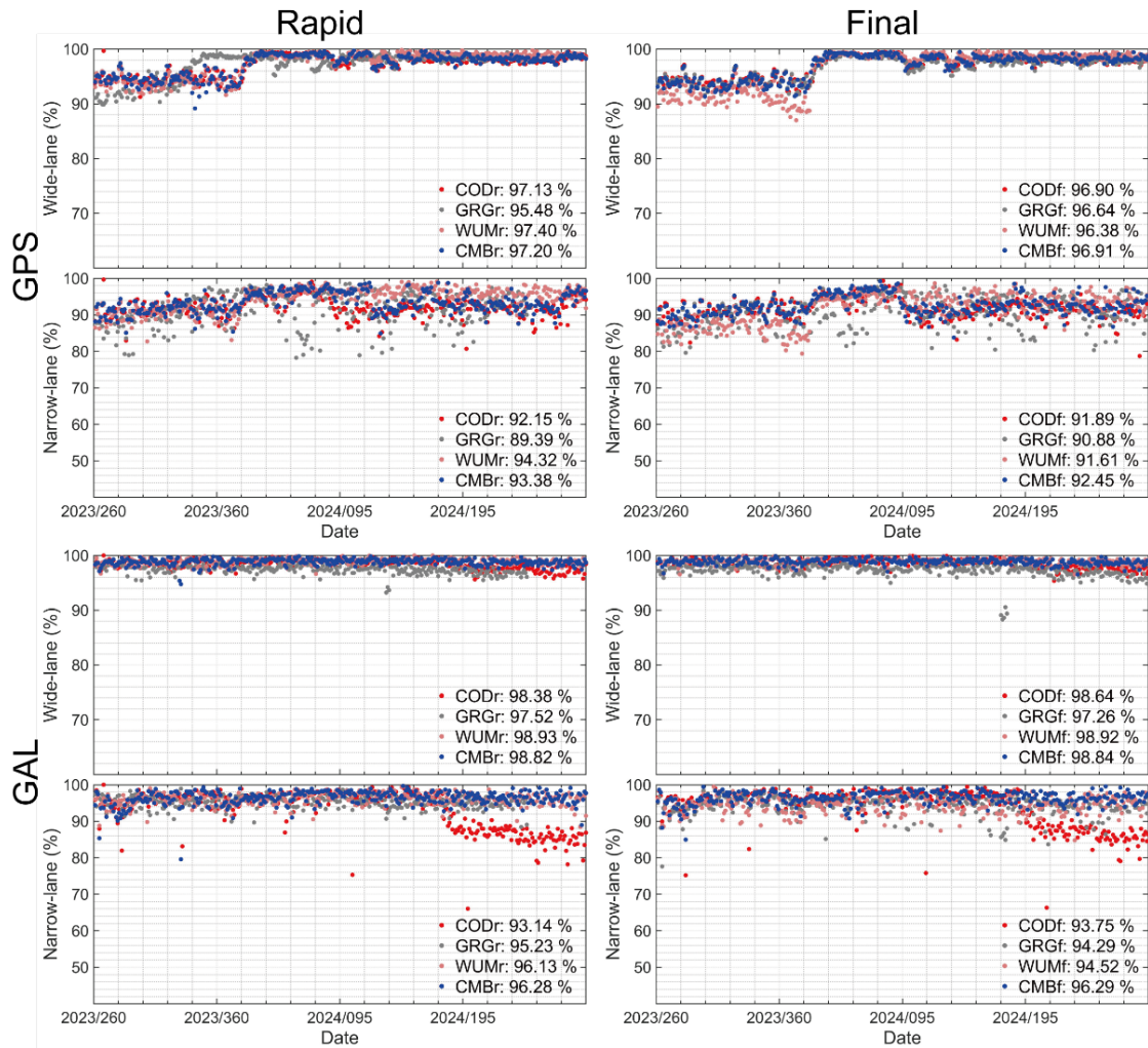
Figure 11: Ambiguity fixing rates for PPP-AR static solutions
