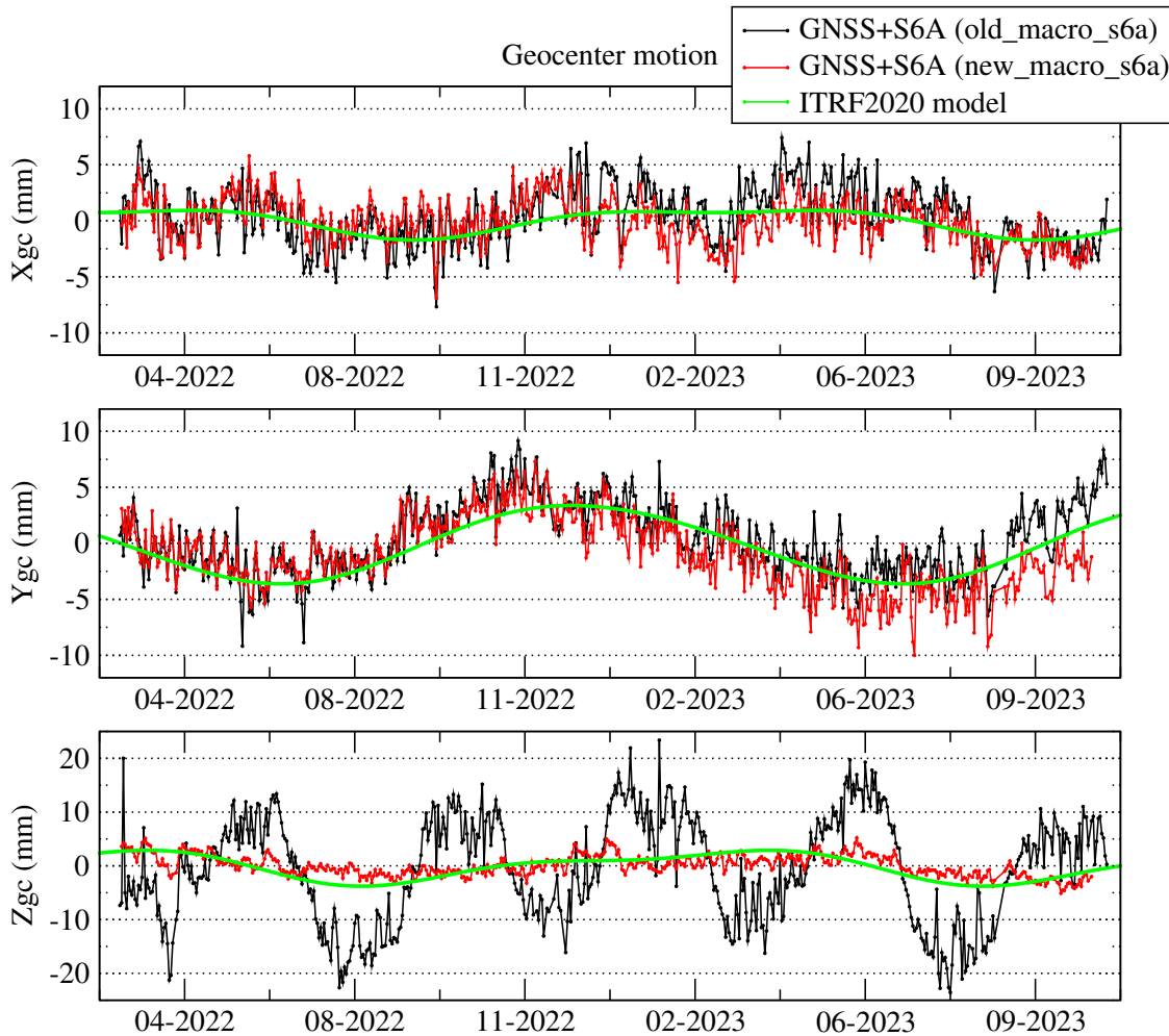
Figure 3: Geocenter motion values as calculated from the GNSS+S6A processings and ITRF2020
