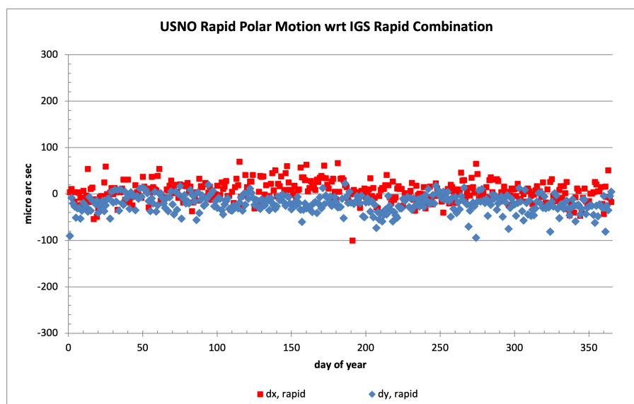
Figure 3: USNO Rapid Polar Motion estimates differenced with IGS Rapid Combination values, 2024.
