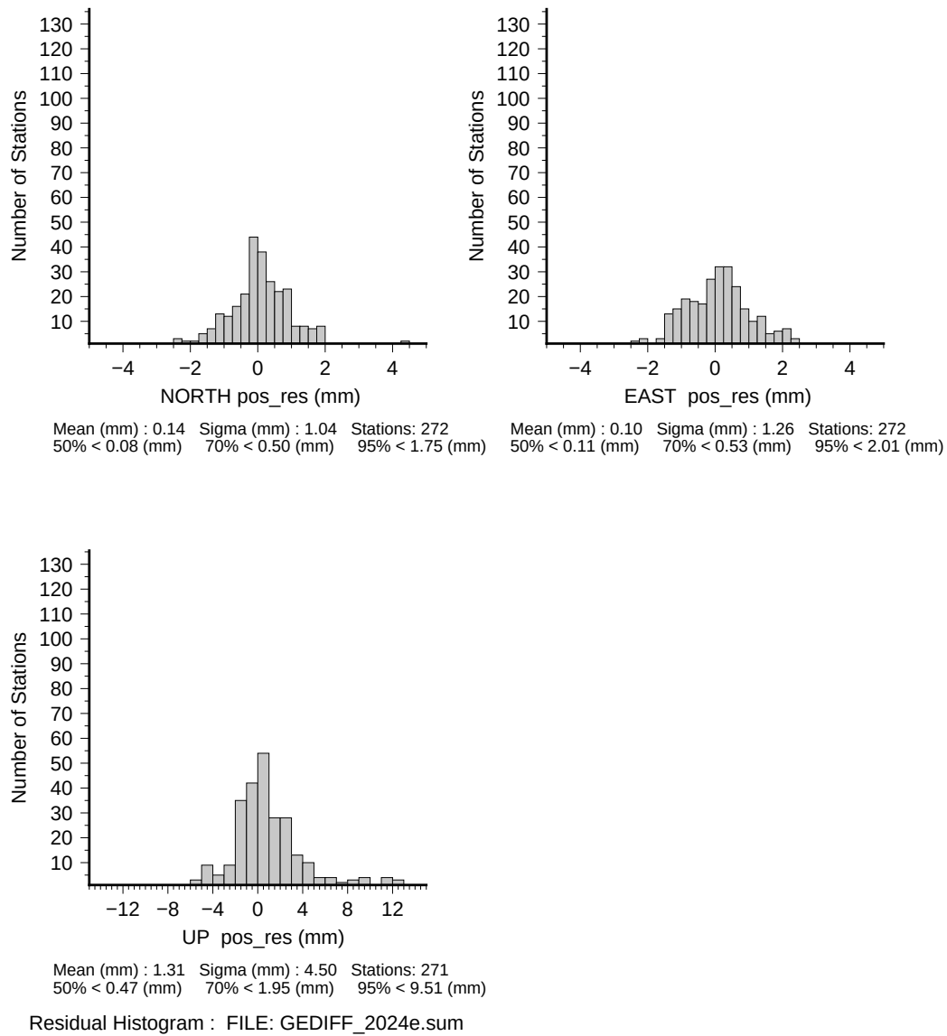
Figure 5: Histograms of the mean differences in North, East, and Height between GPS-only and Galileo-only analyses. The mean differences are small, and the slight positive mean difference in the height component is due to positive height differences for sites with only G01 and G02 antenna calibrations (see Table 6). Large negative height differences occur with fully calibrated antennas in general. Large negative and positive differences in horizontal components occur for fully calibrated antennas.
