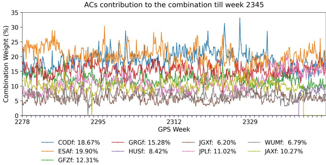
Figure 6: ACs contribution to the Final products combination from week 2278 to 2345
