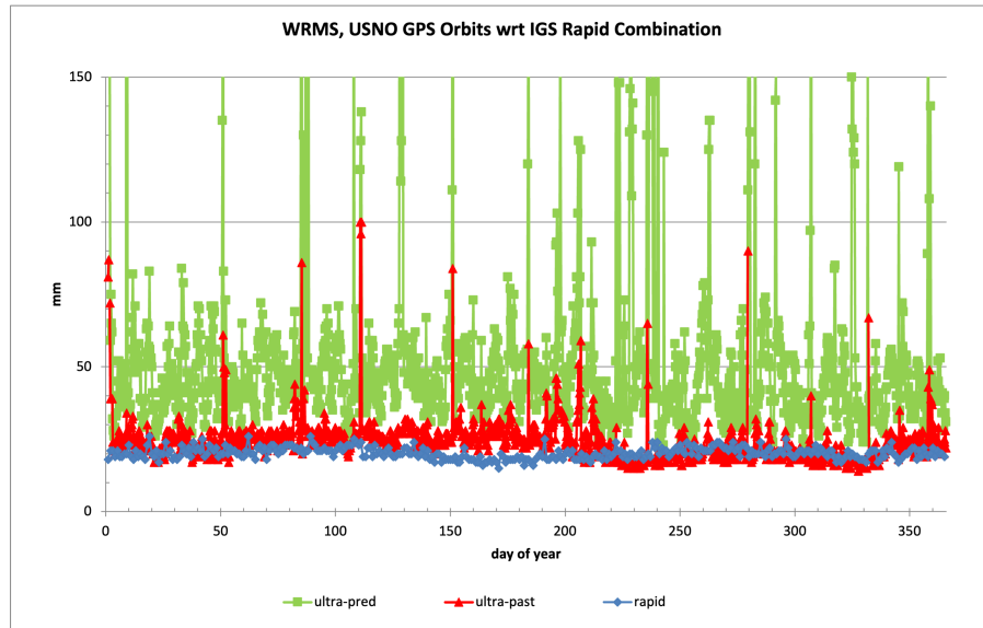
Figure 1: Weighted RMS of USNO GPS orbit estimates with respect to IGS Rapid Combination, 2024. “Ultra-past” refers to 24-hour post-processed section of USNO Ultra-rapid orbits. “Ultra-pred” refers to first six hours of Ultra-rapid orbit prediction.
