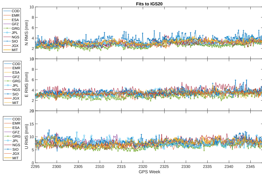
Figure 4: WRMS scatters of the fits to the IGS20 system using typically 45–50 stations. Not all centers used the IGS20 system for the whole year. Note the scales here are twice those used in Figure 3.
