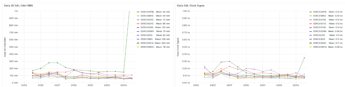
Figure 1: Agreement of real time Galileo orbits (left) and clock (right) products provided by different RT ACs.
