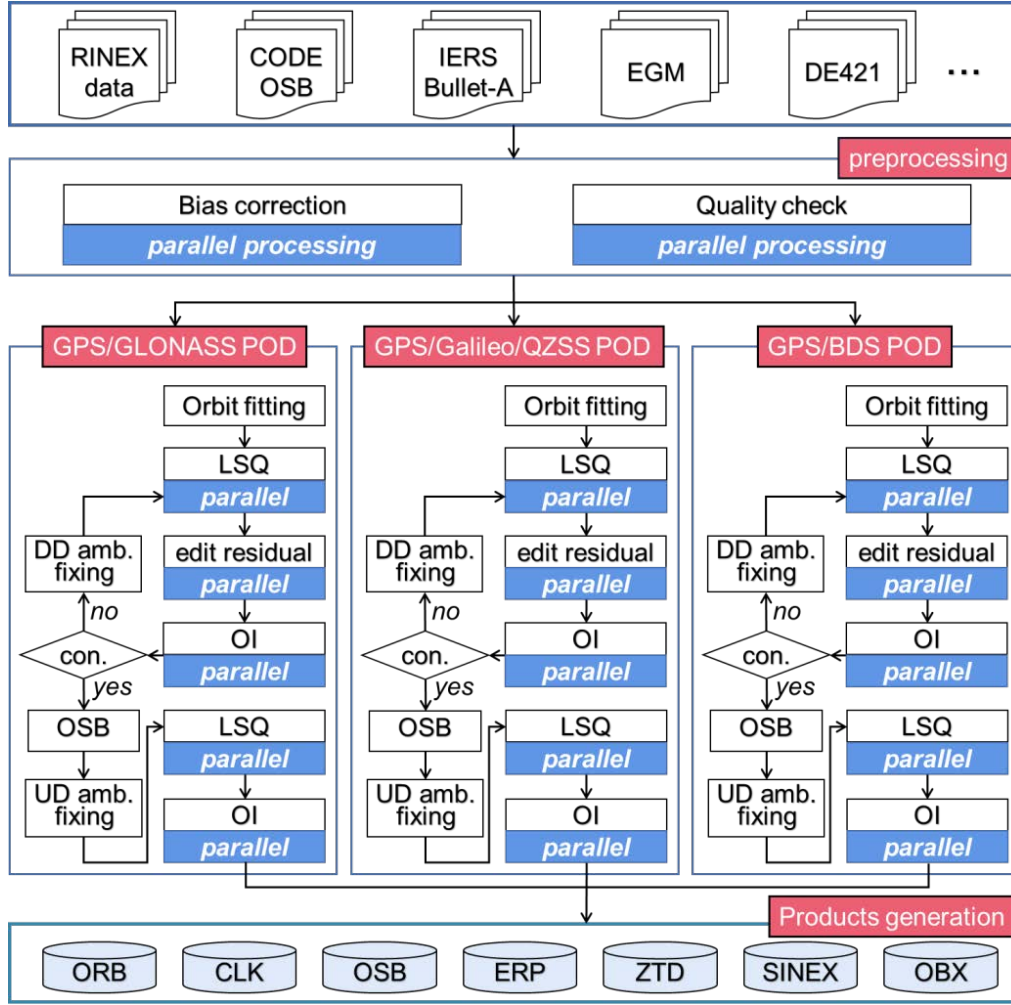
Figure 1: The workflow for the determination of the WUM NRT products.
