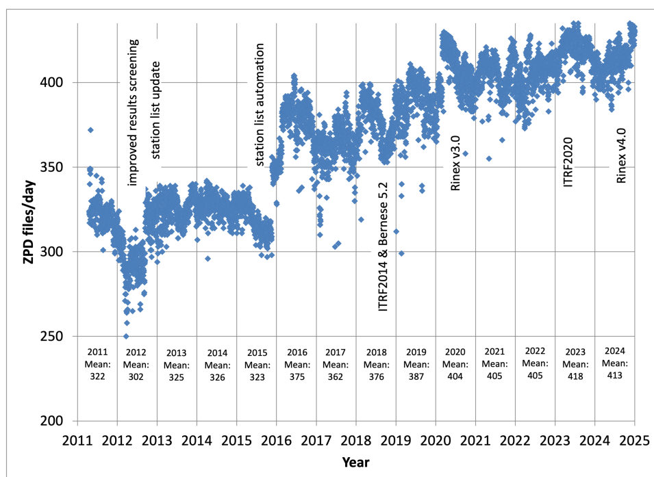
Figure 1: Number of IGS receivers for which USNO produced IGS Final Troposphere Estimates, 2011–2024.
