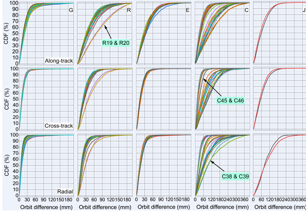
Figure 2: CDFs of real-time orbit precision for GPS, GLONASS, Galileo, BDS and QZSS IGSO and MEO satellites.
