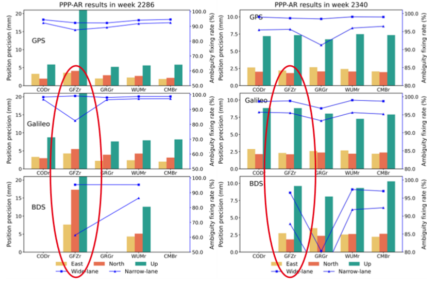
Figure 4: A comparison of GFZ MGEX PPP-AR performance between week 2286 and 2340
