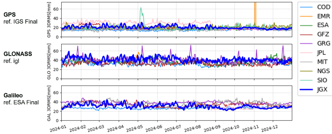
Figure 2: 3D RMS error of final products w.r.t. IGS final (GPS, GLONASS) and ESA final (Galileo) in 2024.
