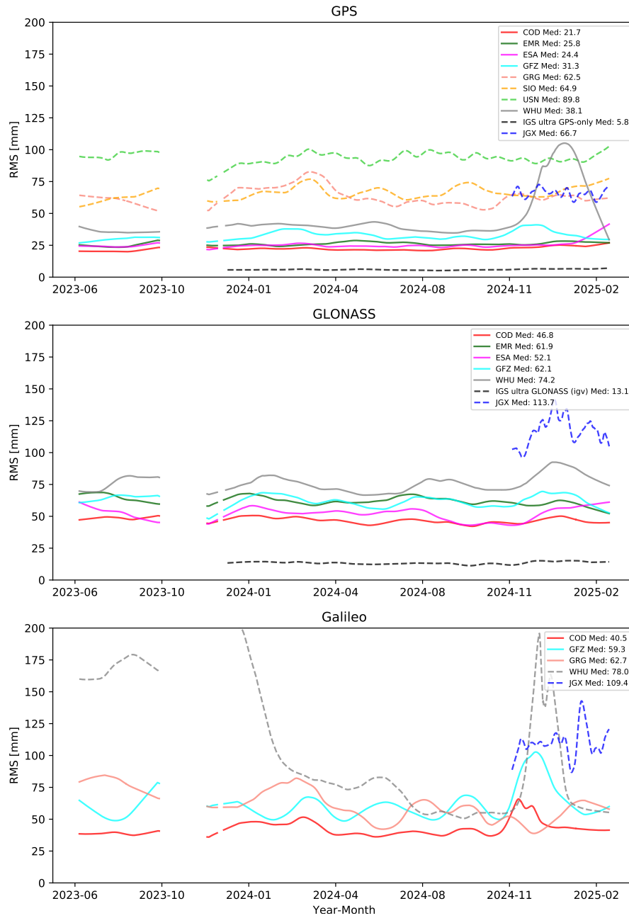
Figure 10: RMS of analysis center orbit solutions (smoothed) compared to the IGS combined orbits for the IGS multi-GNSS ultra-rapid demonstration products for GPS (top), GLONASS (middle) and GALILEO (bottom). The dashed lines are the AC solutions that are not weighted in the combinations, while the solid lines are the weighted ACs.
