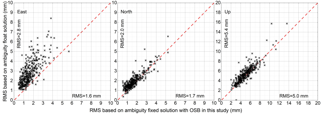
Figure 3: RMS of static PPP solutions with respect to IGS weekly solutions.
