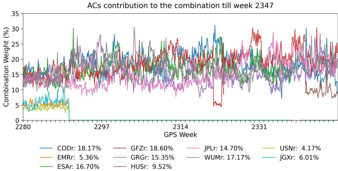
Figure 7: ACs contribution to the Rapid products combination from week 2278 to 2347
