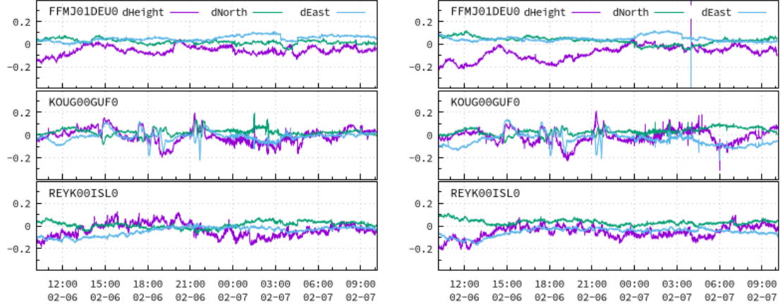
PPP Displacements[m] BNC with SSRA02IGS1 - (C) BKG PPP Displacements[m] BNC with SSRA03IGS1 - (C) BKG
