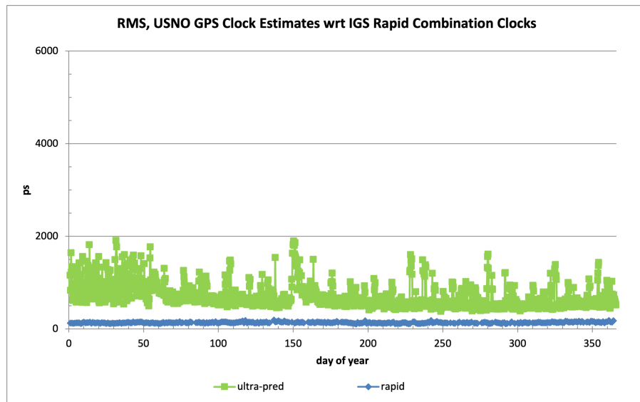
Figure 2: RMS of USNO GPS Rapid clock estimates and Ultra-rapid clock predictions with respect to IGS Rapid Combination, 2024.
