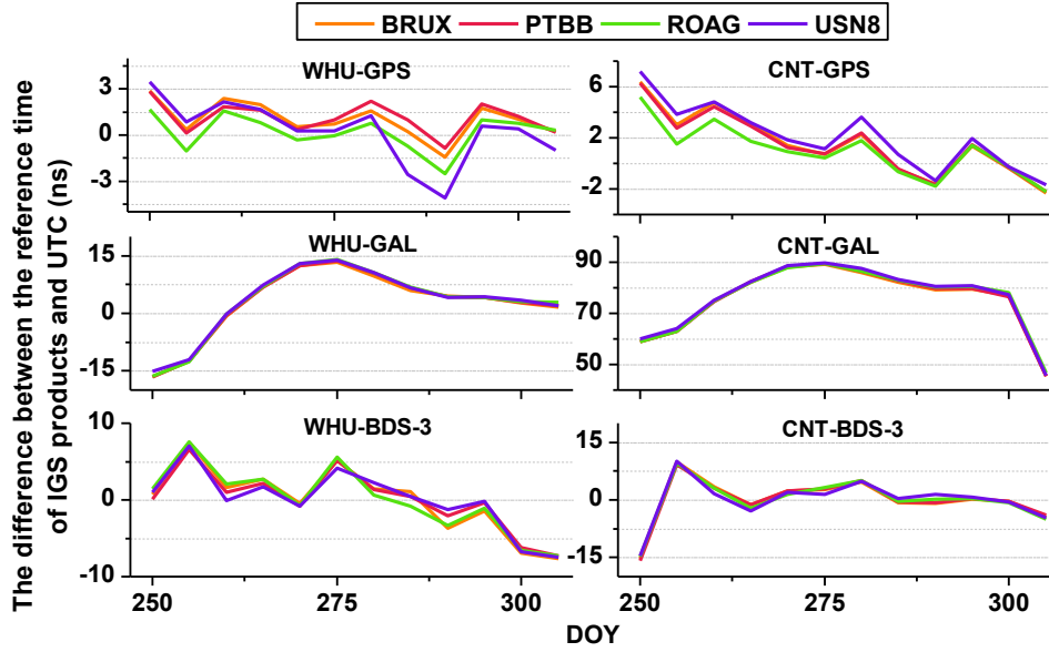
Figure 6: Estimated offset of GPS, Galileo and BDS real-time reference time from UTC using a subset of UTC(k).
