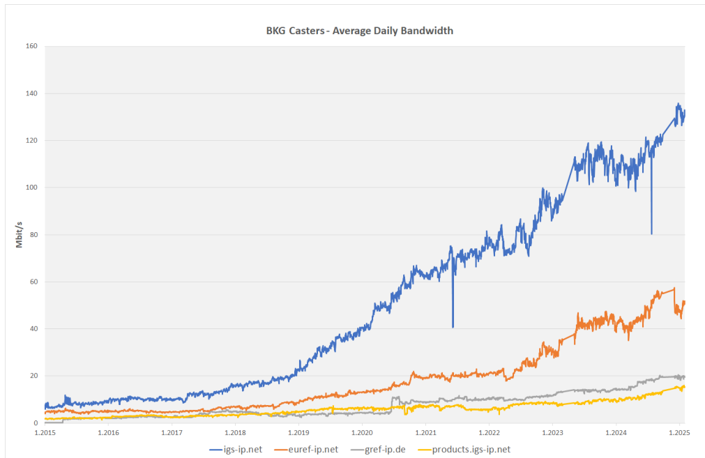
Figure 1: Average daily bandwidth of the BKG Broadcasters from 2015 to the end of 2024
