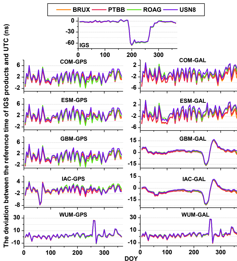
Figure 4: Estimated offset of GPS and Galileo reference time from UTC using a subset of UTC(k) stations, the top panel shows the offset of the IGST timescale with respect to UTC.
