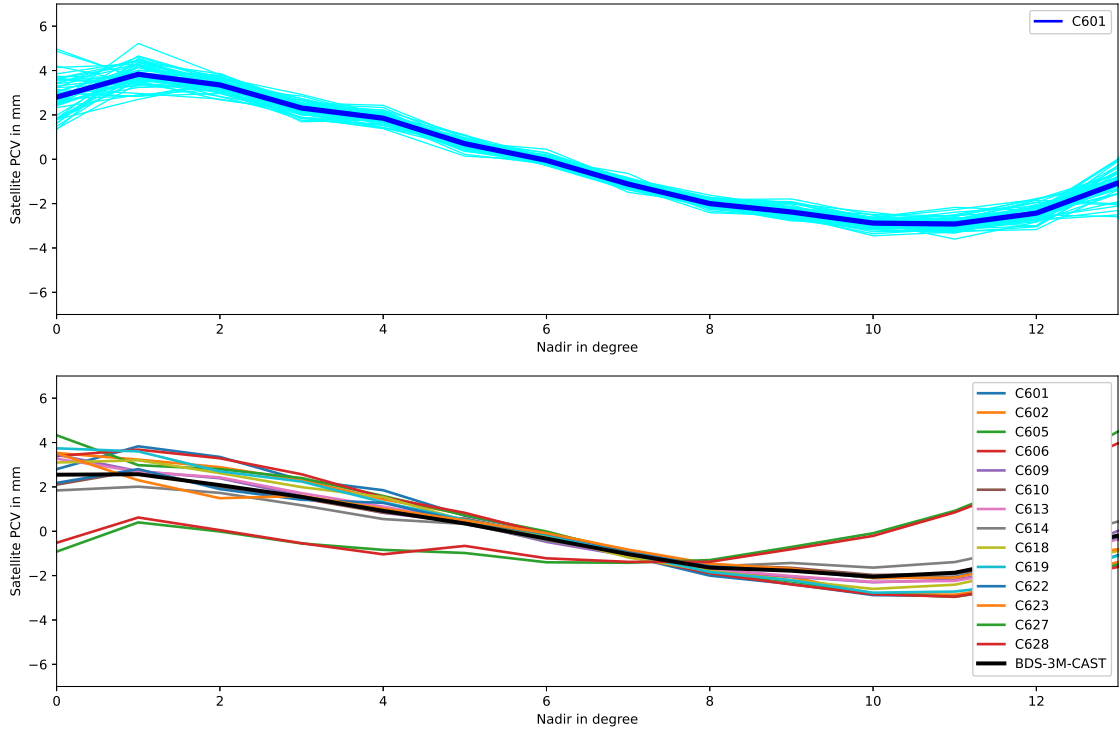
Figure 4: Antenna phase center variations derived from weekly solutions (in cyan) and the averaged value (in blue) for BeiDou satellite C19 (601, type CAST). Below, annual averages of the antenna phase center variations of the BeiDou CAST satellites.
