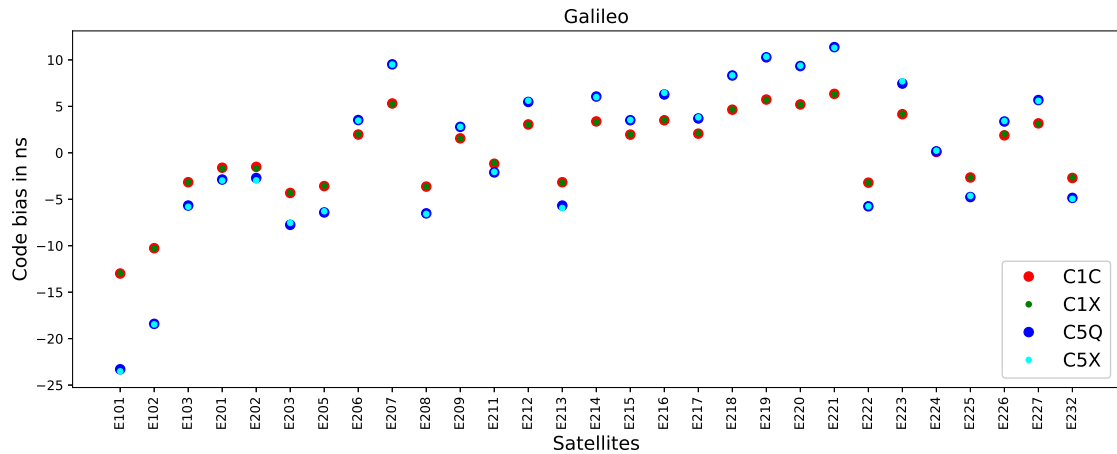
Figure 3: Observable-specific code bias (OSB) estimates for Galileo code observable types (using the RINEX3 nomenclature) and Galileo SV numbers, computed at CODE, for January 2025.
