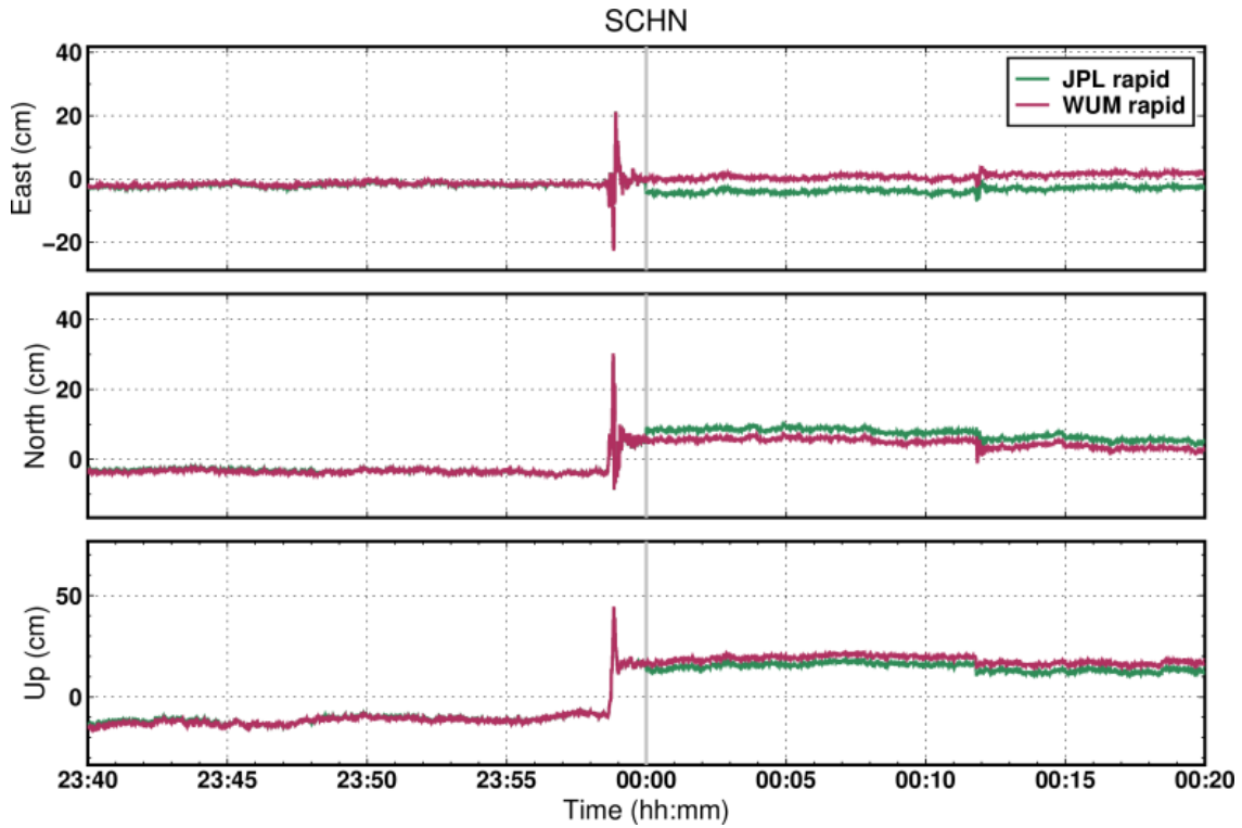
Figure 12: Positioning time series near the earthquake using JPL0OPSRAP and WUM0MGXRAP products (Only GPS used).
