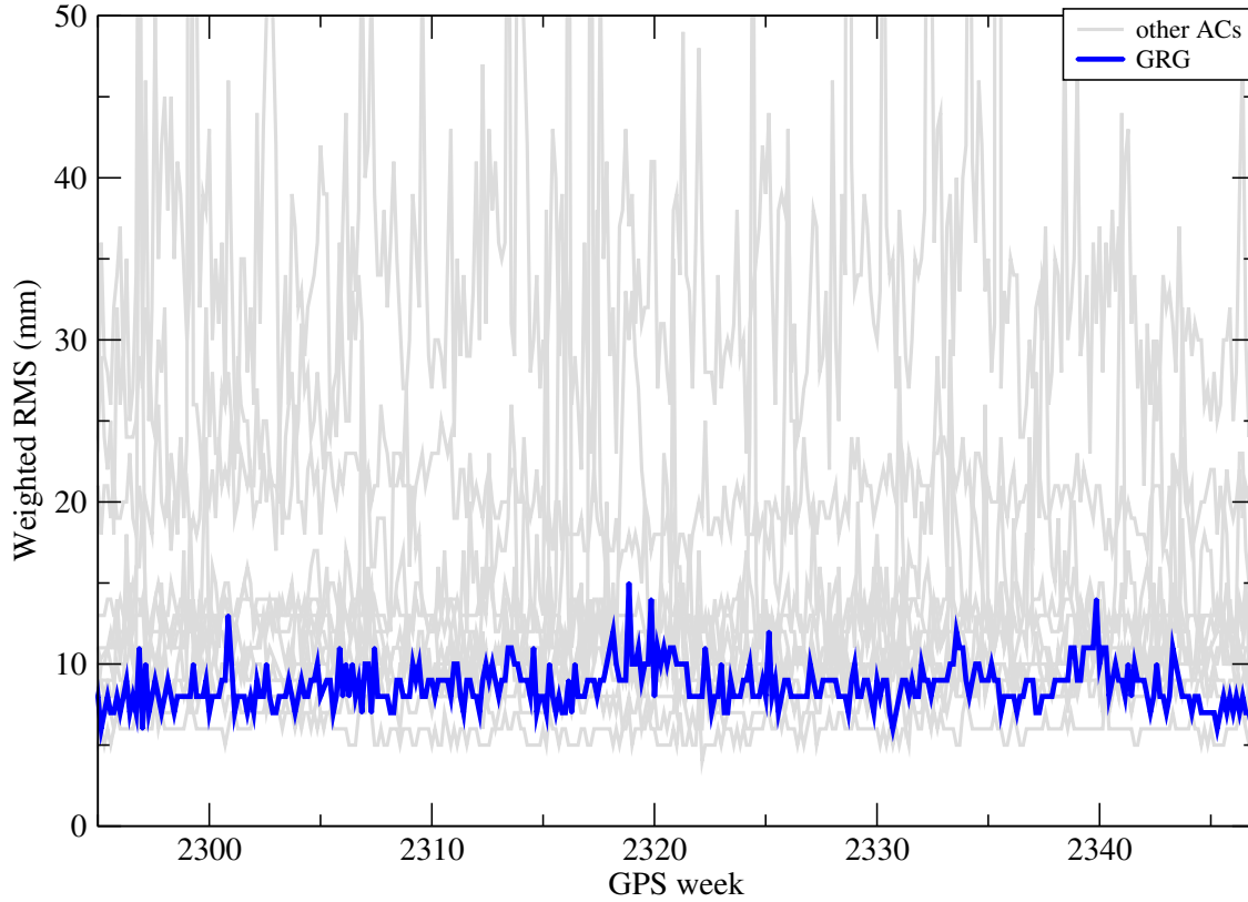
Figure 1: Combination weighted RMS values of the rapid products
