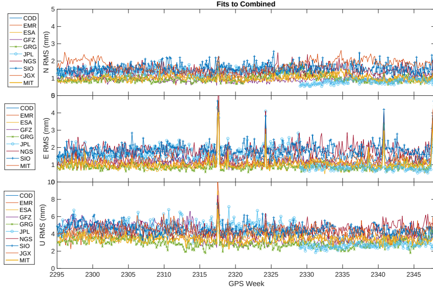
Figure 3: WRMS scatters of the fits of the different IGS ACs to the MIT00PSSNX combined solution for 2024. Not all centers have adopted the IGS20 system for the whole year. Specifically, JPL was weighted only after its adoption of IGS20 models for their finals processing. After this adoption, their performance compared to the other centers was excellent. The outlier points were due to non-detected outliers.
