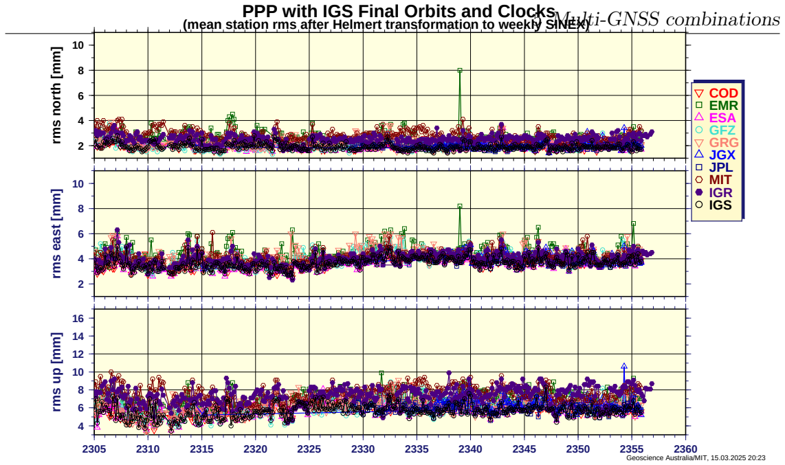
Figure 9: Station RMS residuals from the comparison of the PPP solutions using the final orbit and clock products of each of the analysis centers as well as IGS rapid and final products to the IGS weekly SINEX solution. All PPP solutions were estimated using the same network of IGS20 core sites and using Bernese v5.2 software.
