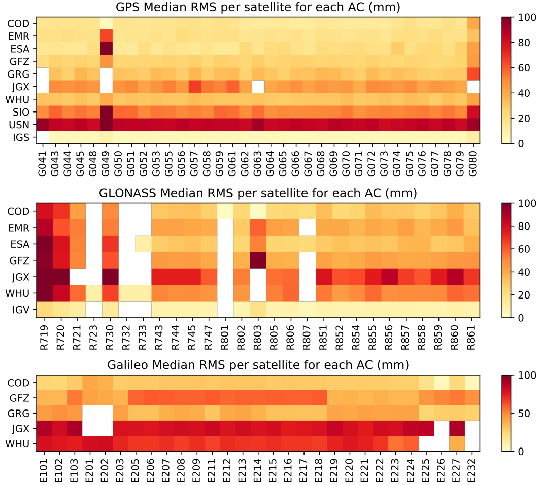
Figure 11: Median RMS of the individual satellites compared to the combined orbits for the multi-GNSS ultra-rapid solutions for GPS (top), GLONASS (middle), and Galileo (bottom). IGS is the IGS ultra-rapid legacy GPS-only combined orbits, and IGV is the current experimental ultra-rapid GLONASS-only combined orbits.
