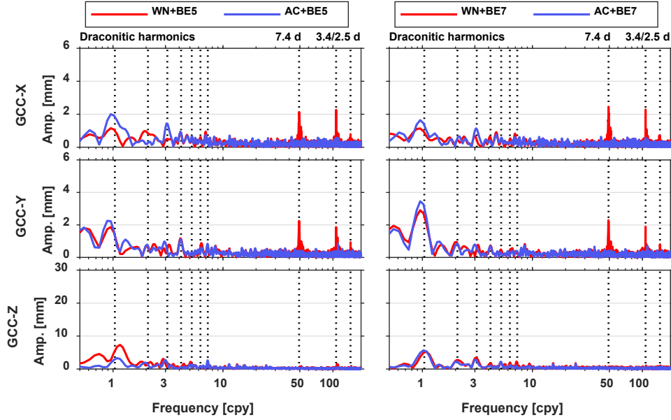
Figure 7: Amplitude spectra of multi-GNSS-derived geocenter coordinates (WN: white noise clock; AC: proposed clock model). BE5 and BE7 represent 5- and 7-parameter ECOM2 models with the a priori box-wing model. The vertical black lines denote the harmonics of a draconitic year and several signals around the 7.4, 3.4 and 2.5-day period.
