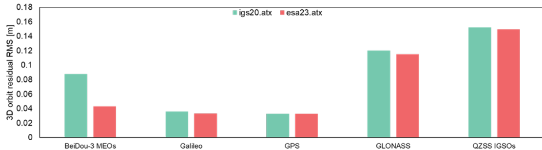
Figure 3: Comparison of day-boundary orbit residual RMS when using igs20.atx and esa23.atx satellite antenna phase center corrections
