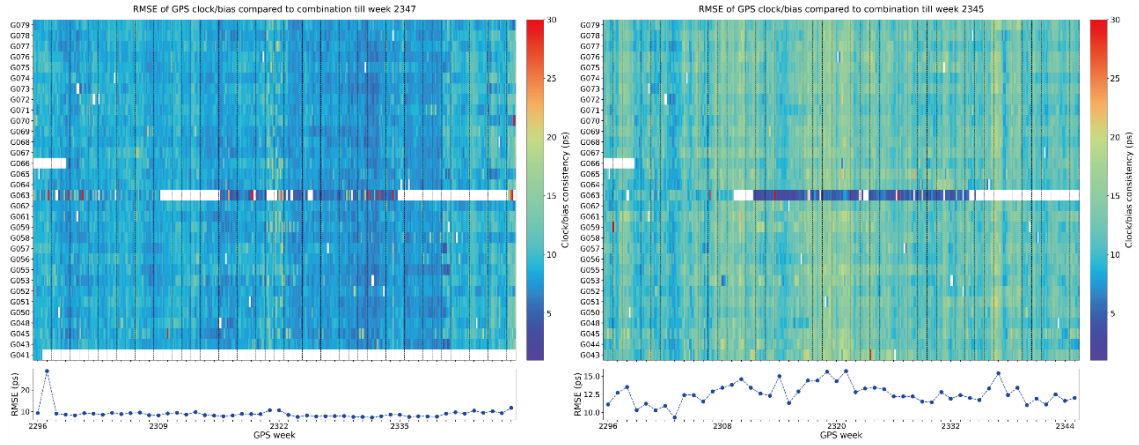
Figure 8: GPS satellite clock/bias combination consistency over the year 2024 (Rapid products for the left panel, Final products for the right panel)
