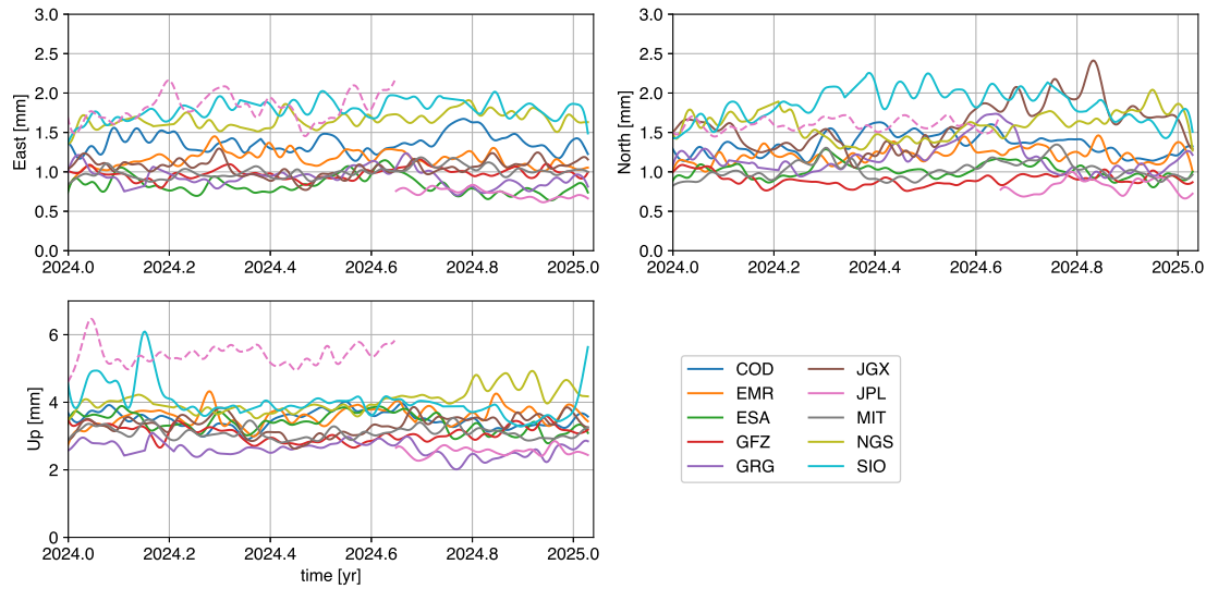
Figure 1: WRMS of AC station position residuals from the 2024 daily IGS SINEX combinations. All WRMS time series are low-pass filtered with a 20 cpy cutoff frequency.
