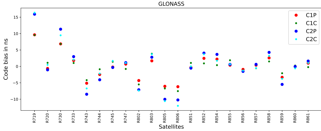
Figure 2: Observable-specific code bias (OSB) estimates for GLONASS code observable types (using the RINEX3 nomenclature) and GLONASS SV numbers, computed at CODE, for January 2025. Note that R719–R747 and R851–R861 correspond to GLONASS-M; R802, R805, R806 correspond to GLONASS-K1 satellite generations; R803 represents the first GLONASS-K2 satellite.
