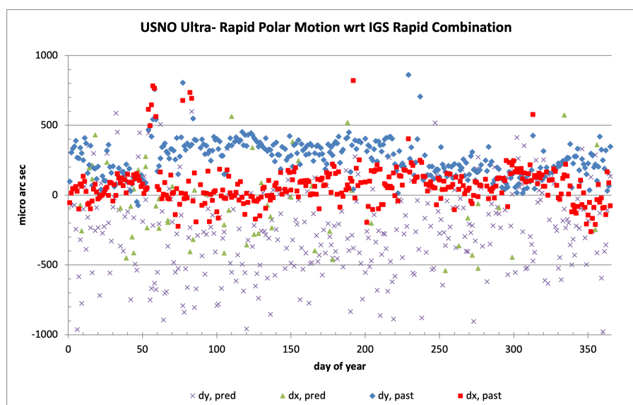
Figure 4: USNO Ultra-rapid Polar Motion estimates differenced IGS Rapid Combination values, 2024. “pred” denotes predicted and “past” denotes post processed.
