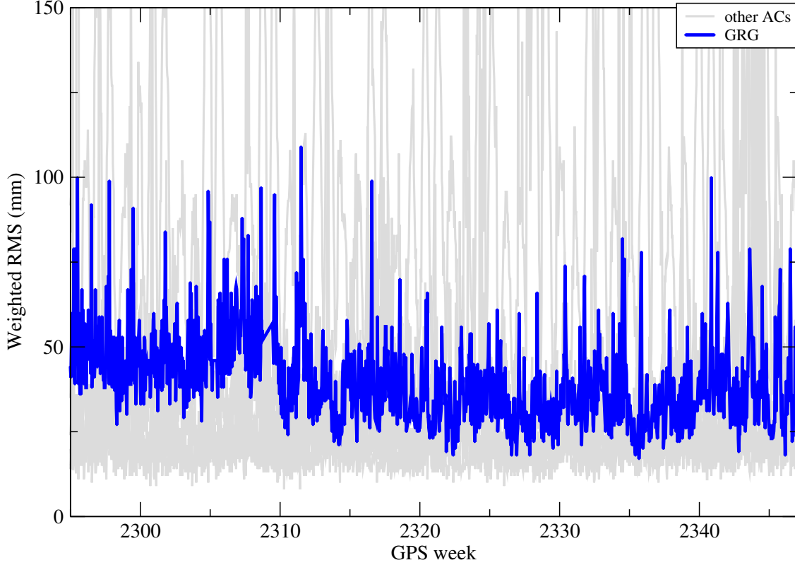
Figure 2: Combination weighted RMS values of the ultra-rapid products
