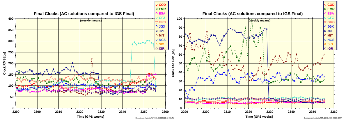
Figure 8: Weighted RMS (left) and standard deviation (right) of IGS final clocks (smoothed). The dashed lines on the figure on the right are the solutions that are unweighted as of February 2025, while the solid lines are the weighted solutions. Note the change in scale of the Y axis.
