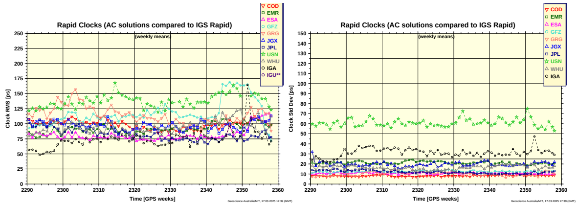
Figure 6: Weighted RMS (left) and standard deviation (right) of ACs rapid clock submissions (smoothed). IGC** are 24-hour products each containing four 6-hour segments from each update interval of the IGS real-time stream. IGU** consists of four separate comparisons to IGR done each day over the first 6 hours of each IGS ultra-rapid product. The dashed lines on the figure on the right are the solutions that are unweighted as of February 2025, while the solid lines are the weighted solutions. Note the change in scale of the Y axis.
