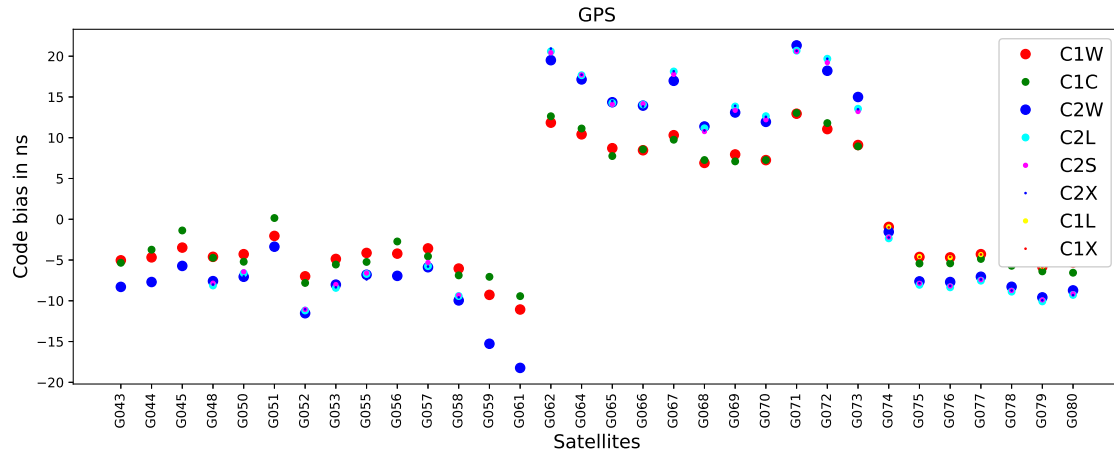
Figure 1: Observable-specific code bias (OSB) estimates for GPS code observable types (using the RINEX3 nomenclature) and GPS SV numbers, computed at CODE, for January 2025. Note that G043–G061 correspond to Block IIR, IIR-M; G062–G073 correspond to Block IIF satellite generations and G074–G080 corresponds to Block IIA.
