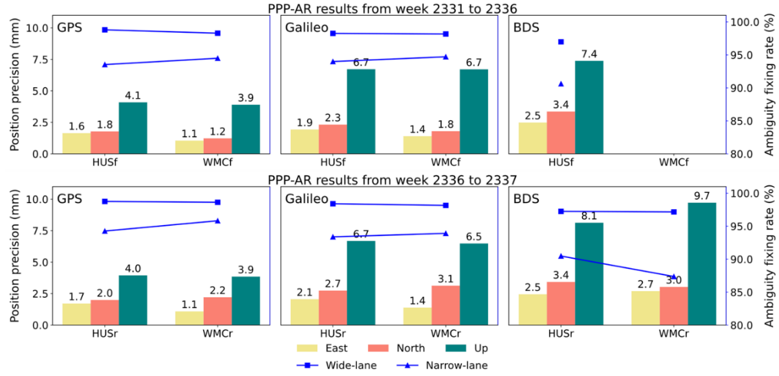
Figure 5: PPP-AR examination of HUS Final and Rapid products.
