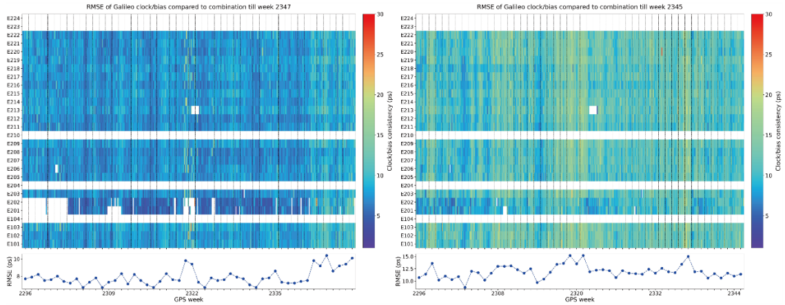
Figure 9: Galileo satellite clock/bias combination consistency over the year 2024 (Rapid products for the left panel, Final products for the right panel)
