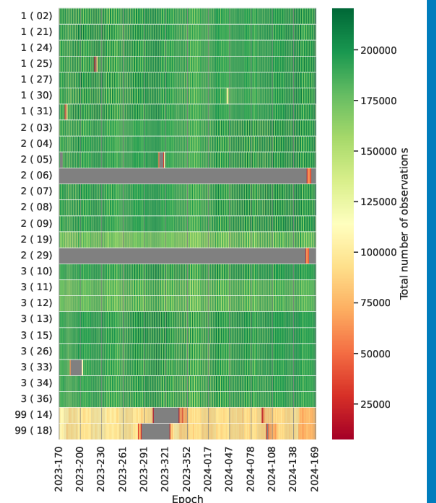
Figure 6: Number of observations for the Galileo constellation included in each daily CODE final solution.
