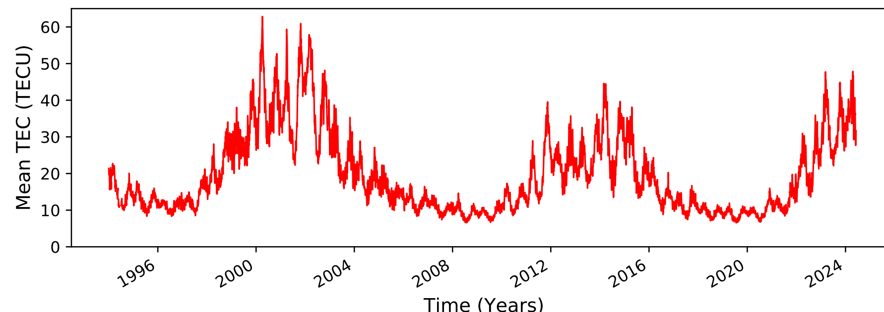
Figure 4: Global mean TEC extracted from the Global Ionosphere Maps (GIMs) produced by CODE. This particular daily time series, meanwhile covering nearly three solar cycles, was created on the basis of hourly GIMs obtained as a by-product from a bias-dedicated GNSS reprocessing effort.
