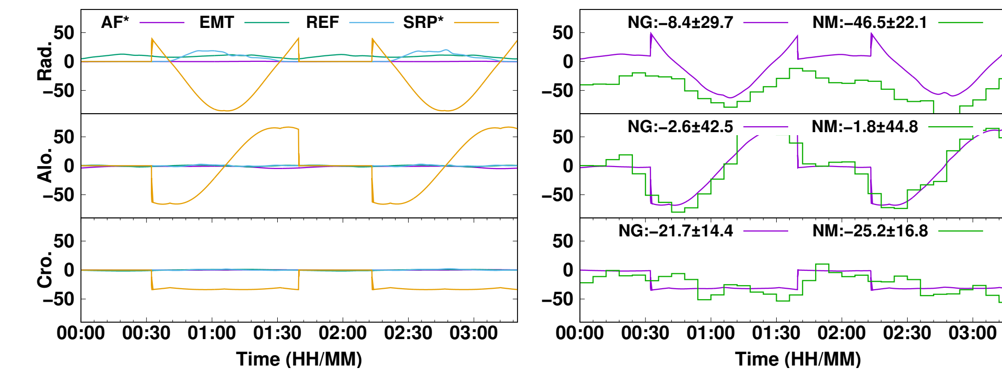
Figure 3: Non-gravitational force modeling for the Sentinel-3A satellite during its first two orbit revolutions on 7/Jun/2018. Left: Each modeled force in the NG orbit solution, SRP and AF are scaled. Right: Comparison between the sum of all modeled forces and the empirical acceleration estimates in the NM solution. Similar trend also happens to the Sentinel-3B satellite. Unit: [nm/s^2] .
