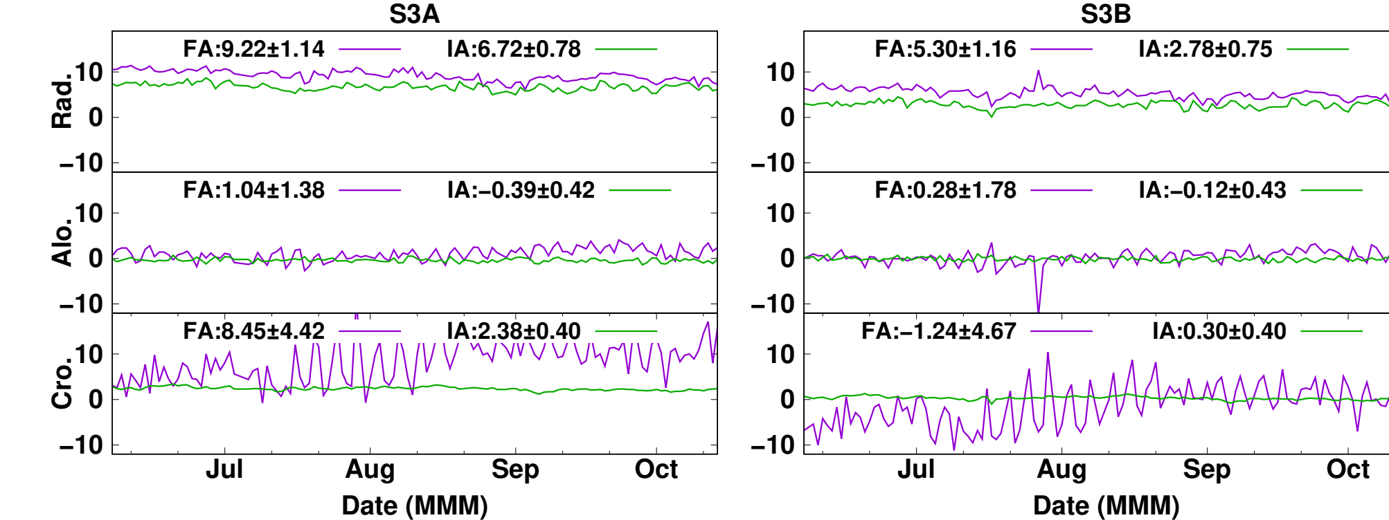
Figure 5: Orbit comparison between the NG orbits and their corresponding kinematic orbit for the two satellites. Unit: [mm].
