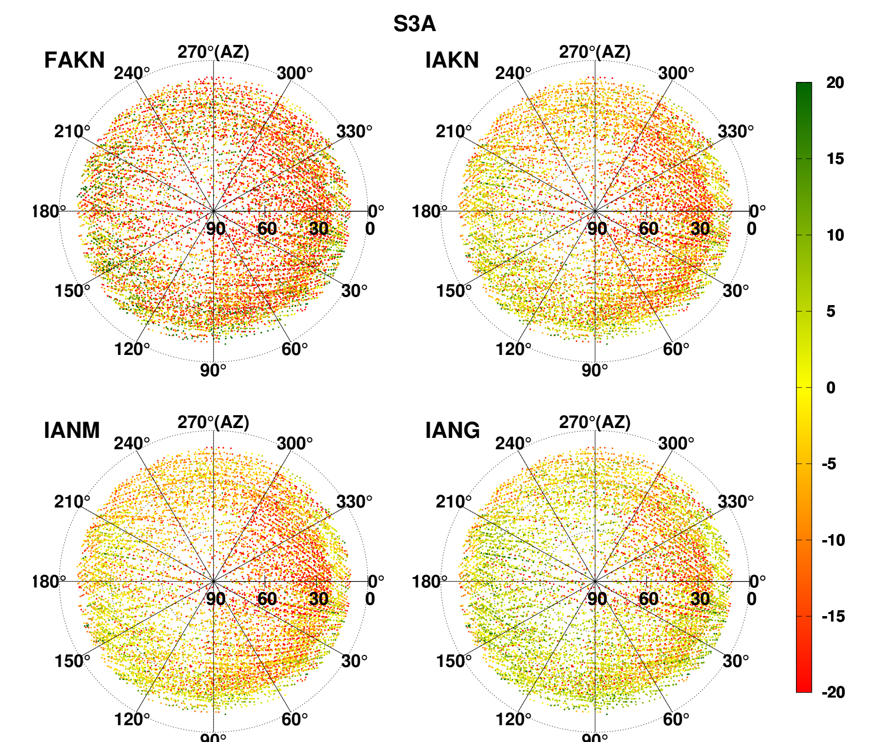
Figure 6: The azimuth- and elevation-dependent SLR residual distributions on sky-plots for the Sentinel-3A satellite. The mean of residuals of the IANG solution is the closest to zero. Similar trend also happens to the Sentinel-3B satellite. Note the reference frame is originated from SLR stations. Unit: [mm].
