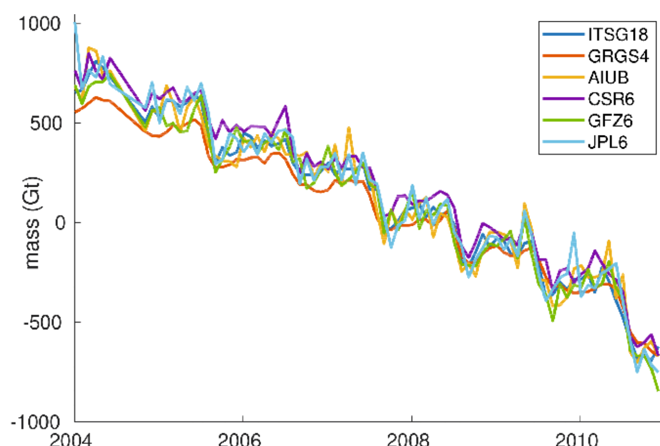
Figure 3: Mass change over Greenland. Only degrees 3 to 90 were taken into account and no Gaussian filter or corrections for leakage and GIA were applied. The attenuated trend in the GRGS-RL04 time-series may be related to the regularization by truncation of the eigenvalues in the inversion step.
