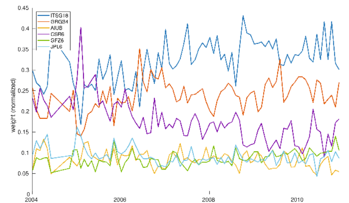
Figure 8: Normalized weights derived with VCE on solution level. These weights are representative for the individual noise levels under the assumption that differences between monthly solutions are dominated by noise, not background model issues.
