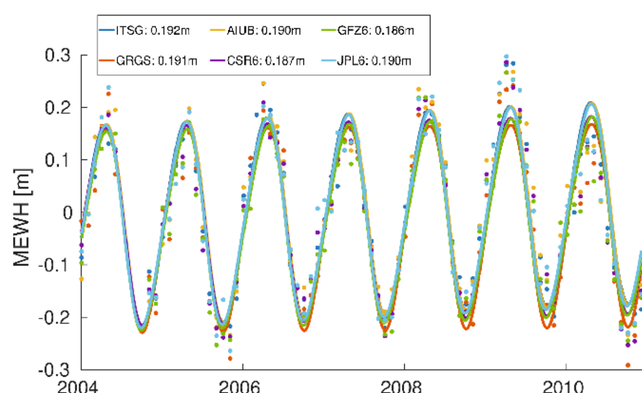
Figure 1: Mean equivalent water heights (MEWH) over the Amazon basin derived from the monthly solutions (dots) and from a posteriori fitted trends and seasonal signals (lines). Annual amplitudes, as given in the legend, agree well with each other.
