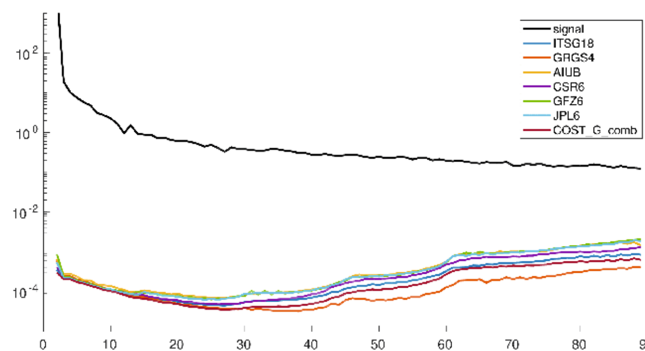
Figure 4: Mean degree variances to a mean model for degrees 2 to 90 including the combination based on VCE on solution level (COST_G_comb). The GRGS-RL04 time-series stands out by its low noise level, related to the regularization applied.
