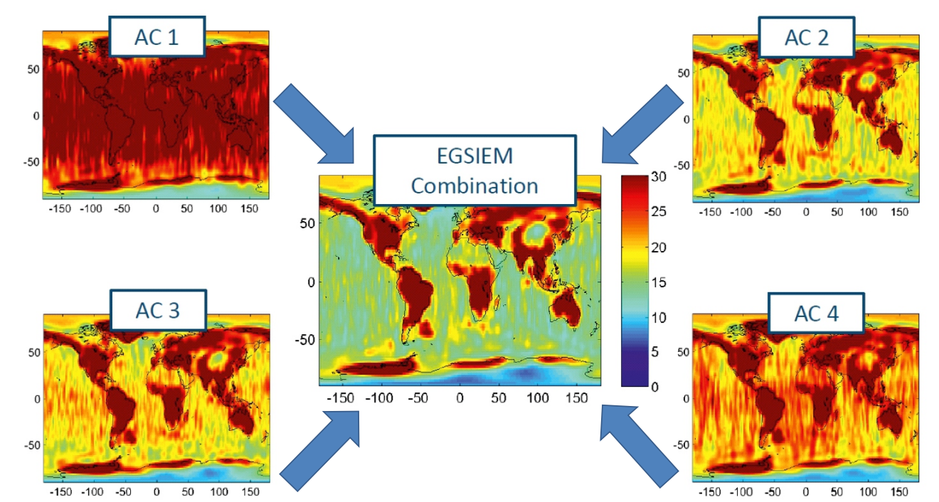
Fig. 6: Noise reduction (visible over oceans) achieved by combination of monthly gravity fields.
