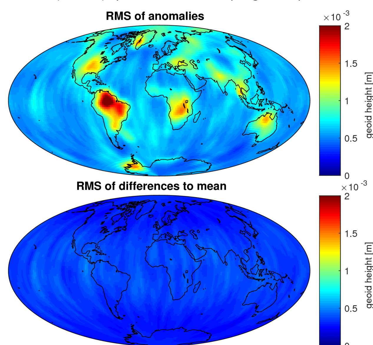
Fig. 4: Spatial distribution of non-secular, non-seasonal signal (anomalies, top) or differences to the arithmetic mean (bottom).
