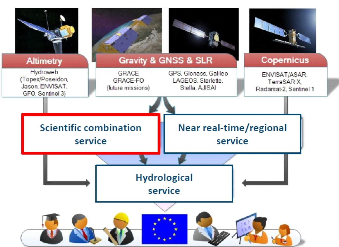
Fig. 1: EGSIM is installing three services related to temporal gravity field variations. The main goal is early warning in case of floods to improve emergency management.
