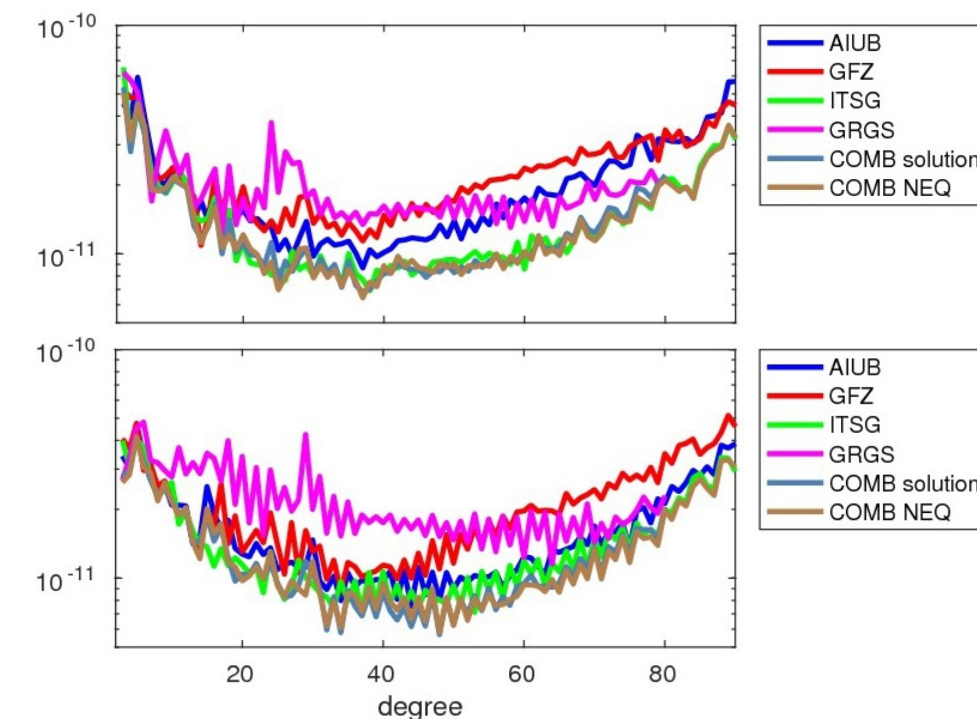
Fig. 8: Degree amplitudes of anomalies of individual contributions and combined monthly gravity fields for January 2006 (top) and June 2006 (bottom).
